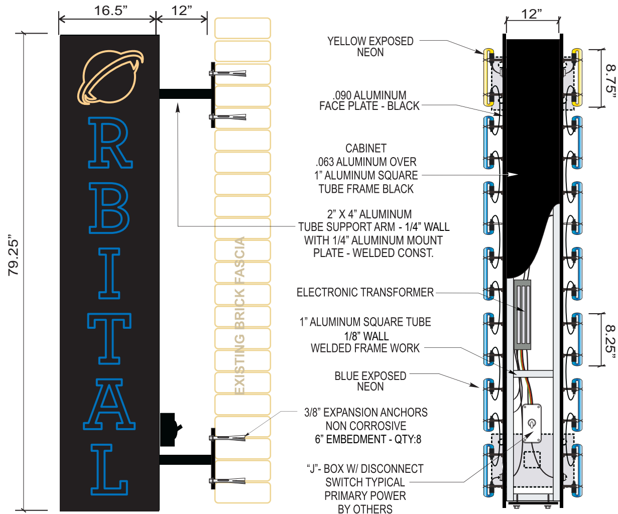
FRONT ELEVATION - Sign Type (1)(QTY:1) D/F Exposed Neon Projecting Sign - Flag Mount Scale: 3/4" = 1' (9 SQFT)
