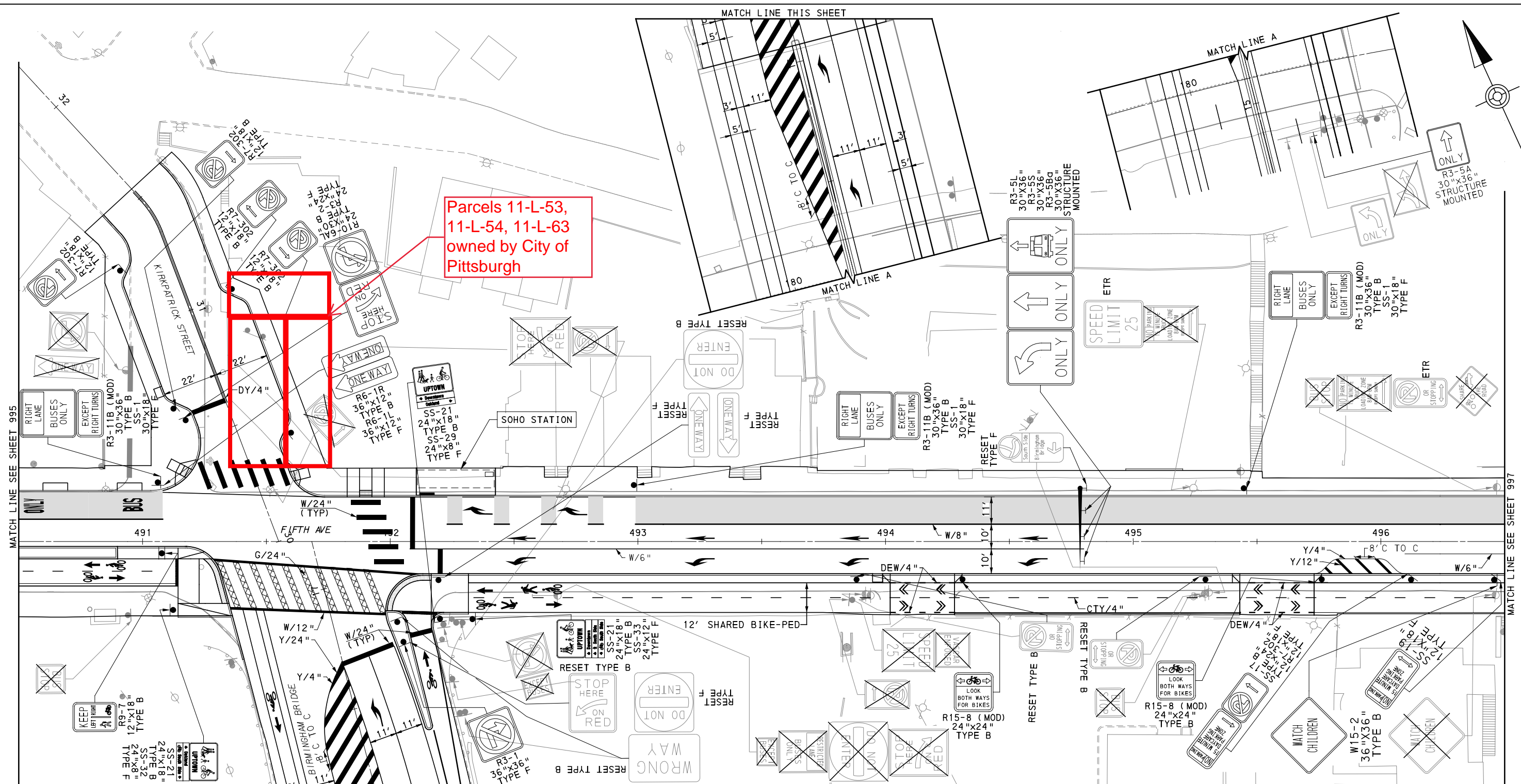
Location Map – Exhibit F – Parcels related to the Kirkpatrick Street Realignment, subject to change as design progresses.
