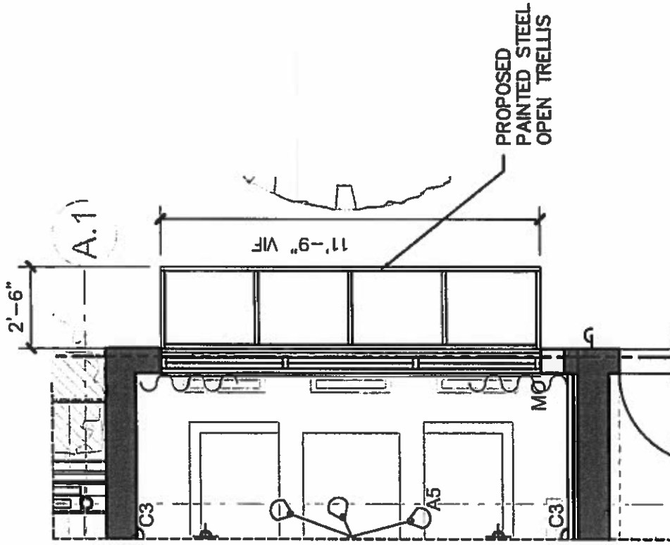
2 TRELLIS RCP-BUILDING 5313 1/4"=1'-0" RE:RCPA2.216
